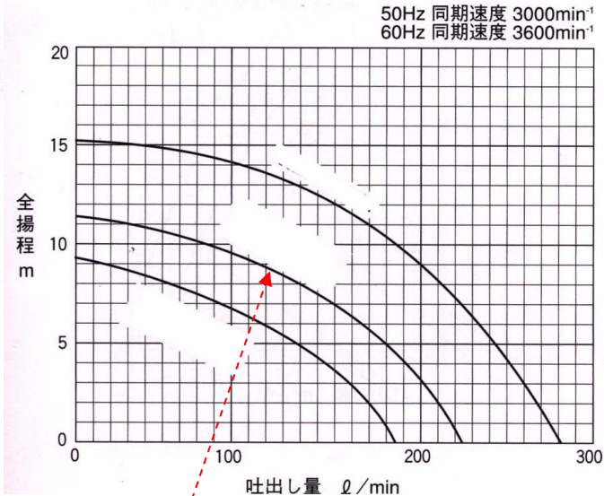
EA345JW-50, -60
