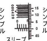
図 C READING 5.005 MM
